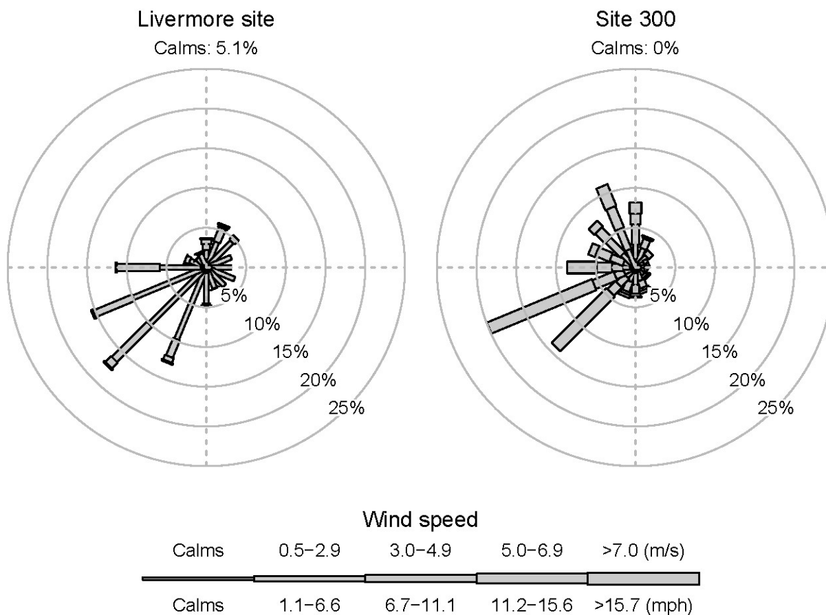
Figure 1-2. Wind roses showing wind direction and wind speed frequencies at the Livermore Site and Site 300 during 2021. The length of each spoke is proportional to the frequency at which the wind blows from the indicated direction. Different line widths of each spoke represent wind speed classes.
