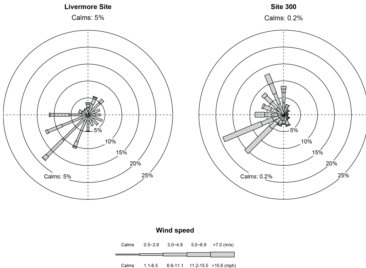
Figure 1-2. Wind roses showing wind direction and wind speed frequencies at the Livermore Site and Site 300 during 2018. The length of each spoke is proportional to the frequency at which the wind blows from the indicated direction. Different line widths of each spoke represent wind speed classes.
